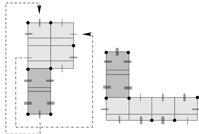
FIGURE 2. Decomposition of a surface into two cylinders
