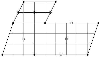
FIGURE 6. Weierstrass points of a two-cylinder surface
