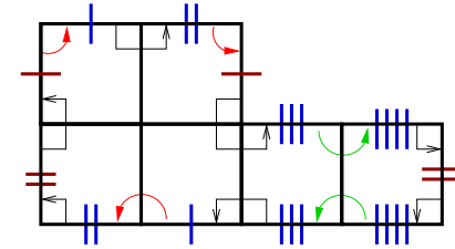
FIGURE 1. Surface with one angle of 6\pi
