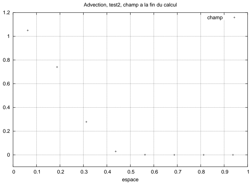
Figure 4 advection, 8 mailles, extrapolation
