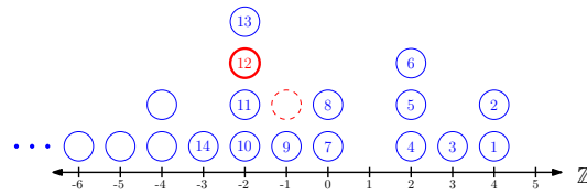
(a) Configuration X
