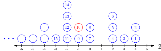
(b) Configuration \Phi_\xi(X) with \xi = 12 .
