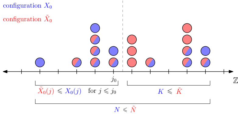
Figure 3.1. Two configurations X_0 (in blue) and \tilde{X}_0 (in red) that satisfy (H2). There are more red balls than blue balls located in \llbracket j_0+1, +\infty \llbracket ( K = 5 \leq 9 = \tilde{K} ) and also more red balls than blue balls in total ( N = 13 \leq 14 = \tilde{N} ) but there are at least as many blue balls than red balls in every bin located at j < j_0 .
