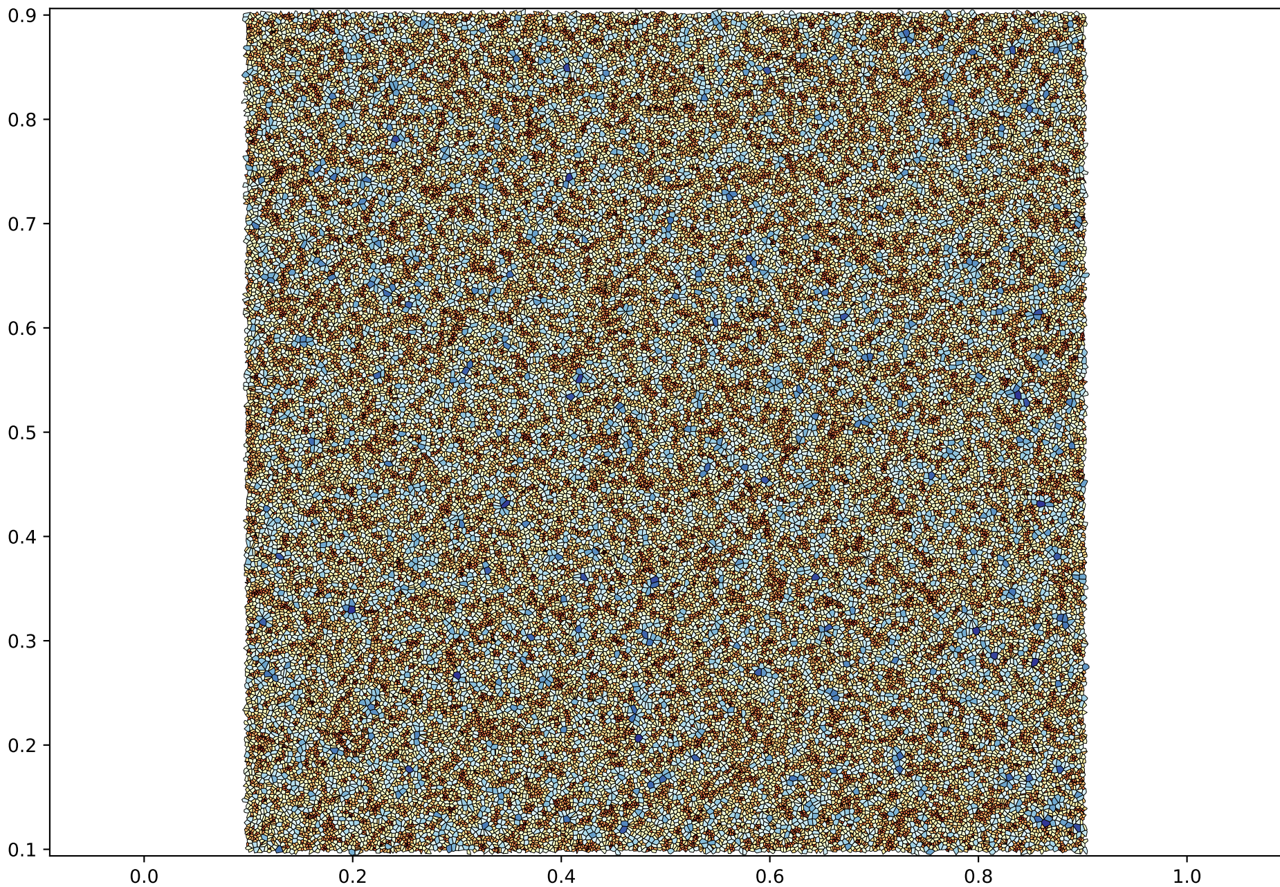
Voronoi heatmap, lambda=100000, a_c=1.2217
